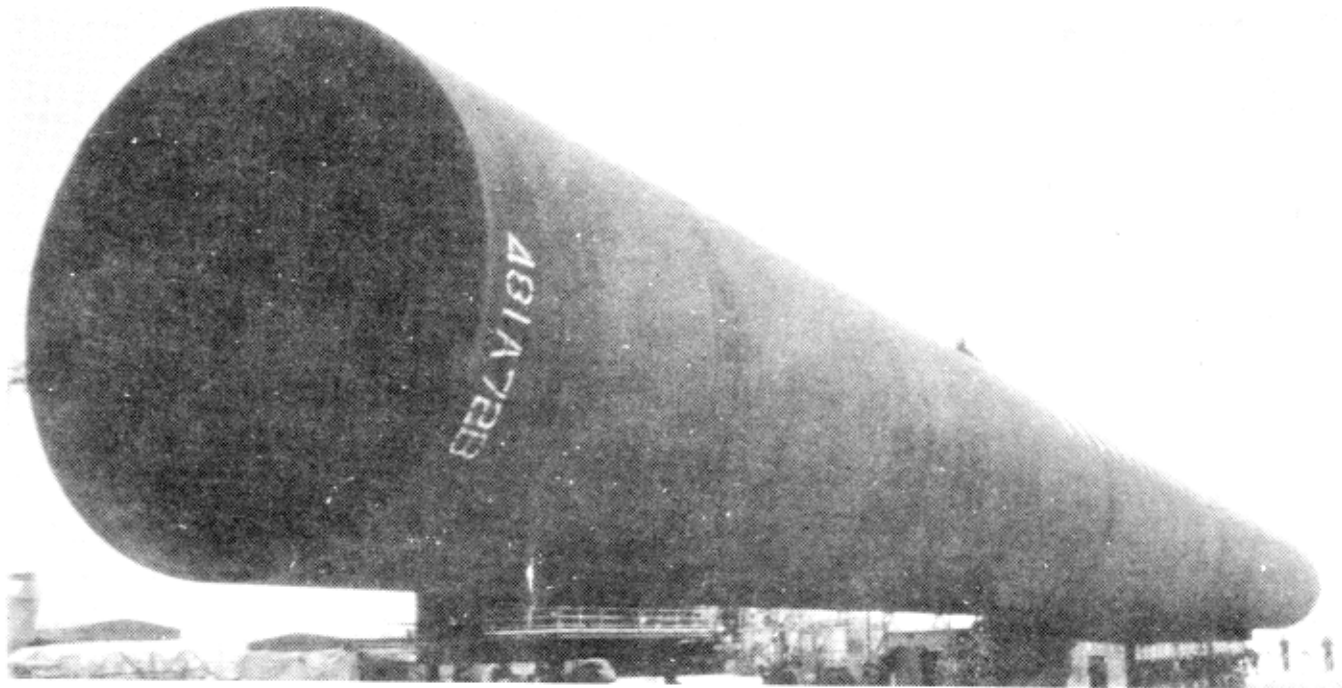
Fig. 1 – 3m dia x 80m long piles were used to support the piers of the Jamuna River Multipurpose bridge in Bangladesh
